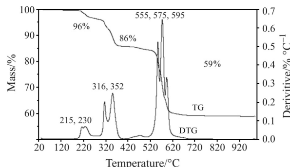
Fig. 3 TG and DTG curves of Na-jarosite
