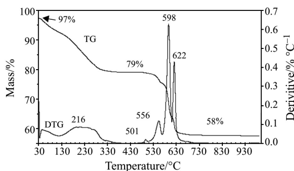
Fig. 1 TG and DTG curves of K-jarosite
