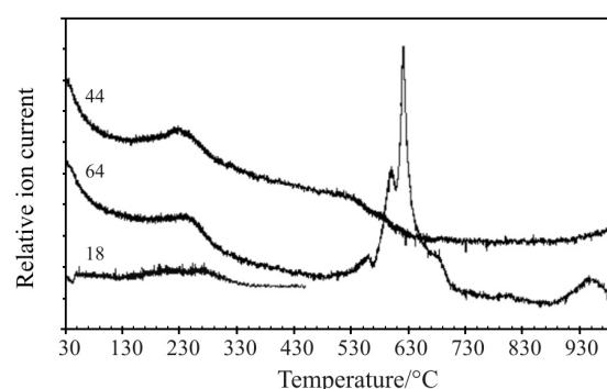
Fig. 2 Relative ion current of evolved gases for the decomposition of K-jarosite
