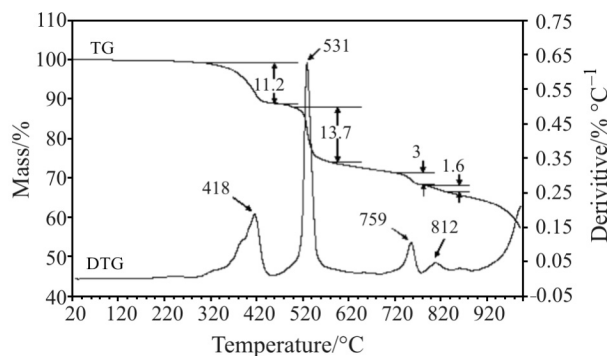
Fig. 4 TG and DTG curves of Pb-jarosite
